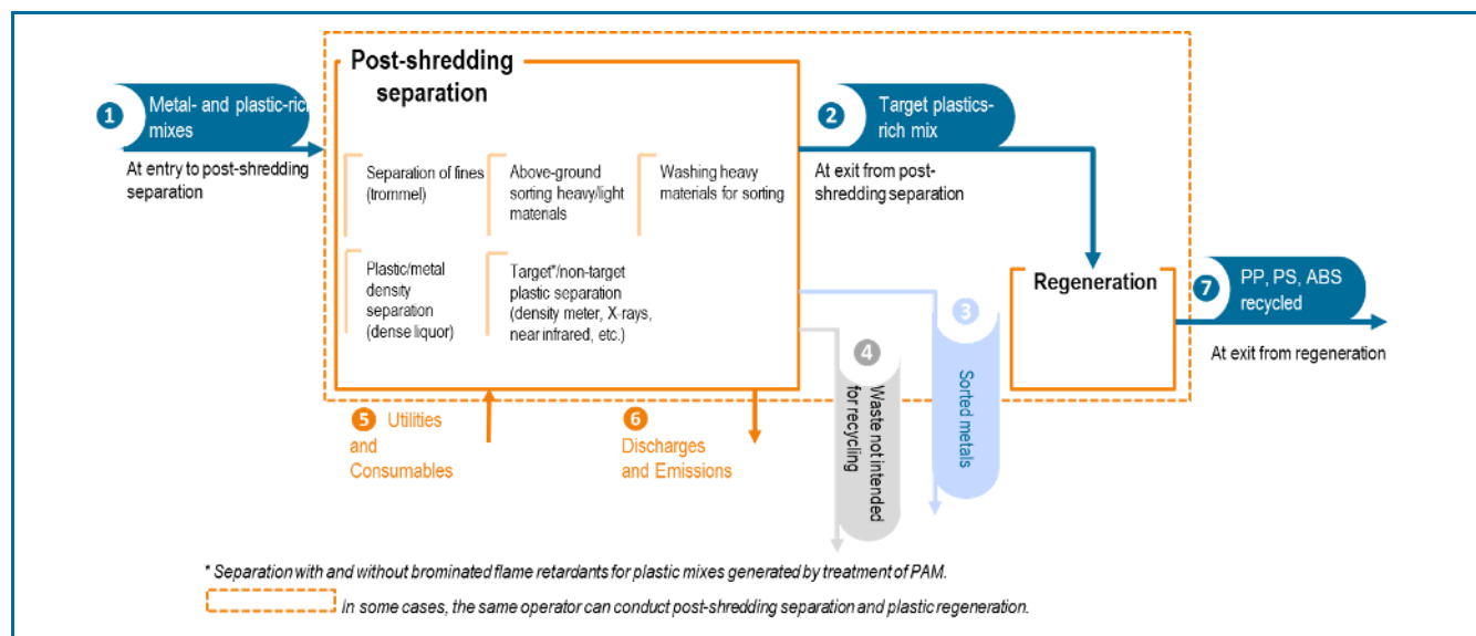
FIGURE 3: EXAMPLE OF SCHEMATIC FIGURE OF A STEP - CASE OF POST-GRINDING SEPARATION OF PLASTIC- AND METAL-RICH MIXES FOLLOWING WEEE PROCESSING
